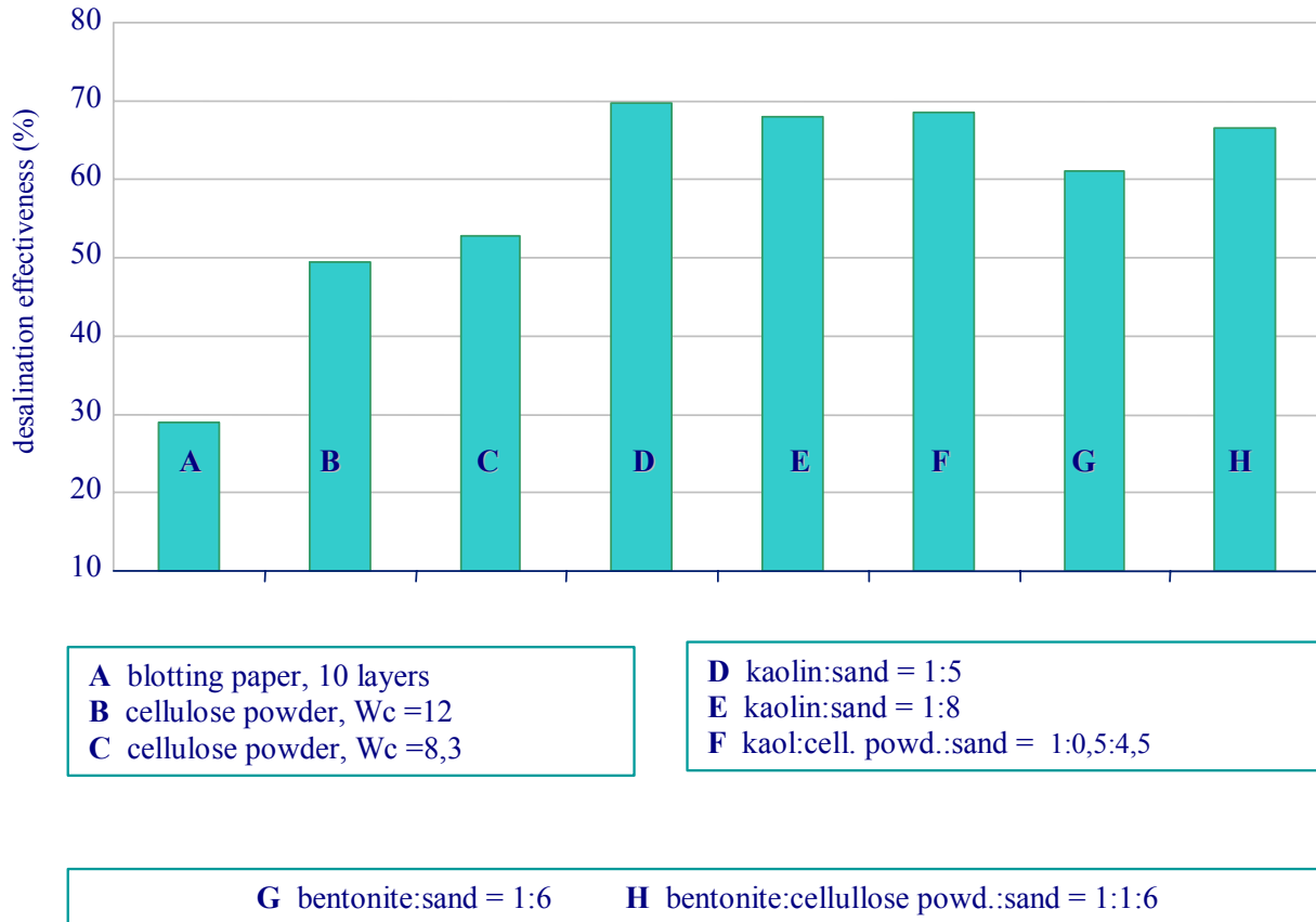
Figure 4: Influence of poultice type on desalination effectiveness of bricks. After Domaslawski et al. 1998 [45]
