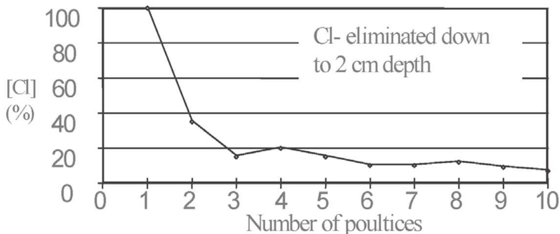
Figure 11: Follow-up of the chloride content during poultice desalination. The authors noticed that desalination was effective only down to 2 cm depth. After Fassina & Molteni, 1994 [16].
