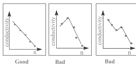
Figure 10: Recommendation for an optimal desalination, according to Ciabach & Sjibinski [75]. n = number of poultices. The curves represent the conductivity of each successive poultice applied to the object. It was proved that even if the “good” evolution is achieved, desalination may not be successful.
